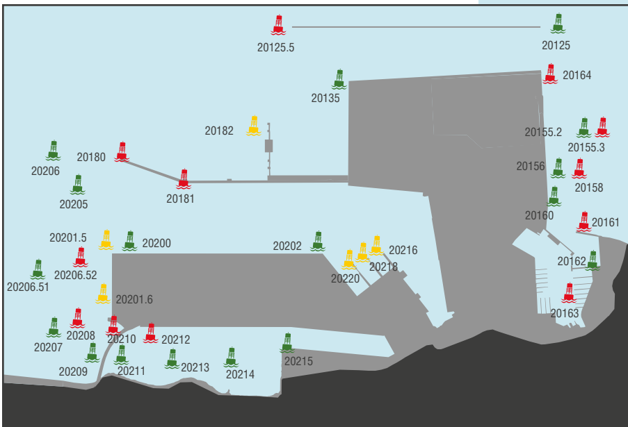
← Layout of Algeciras Port marking system
