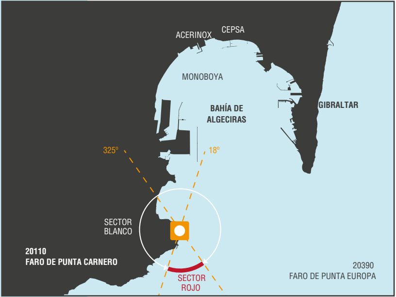
Layout of Bay of Algeciras entry lighthouses
