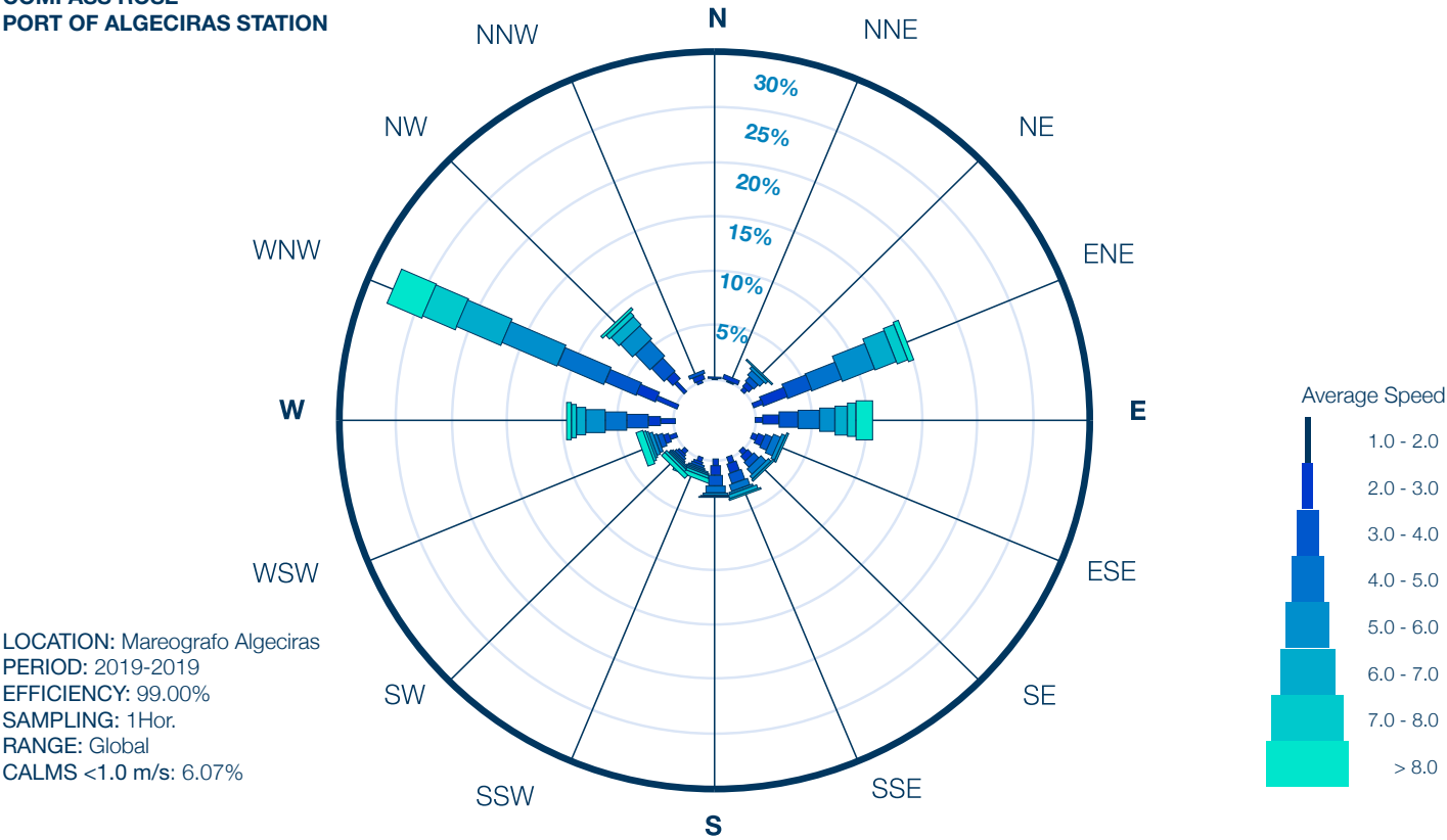
Compass Rose in Port of Algeciras. REMPOR Station (Direction of origin 0=N ; 90=E)
