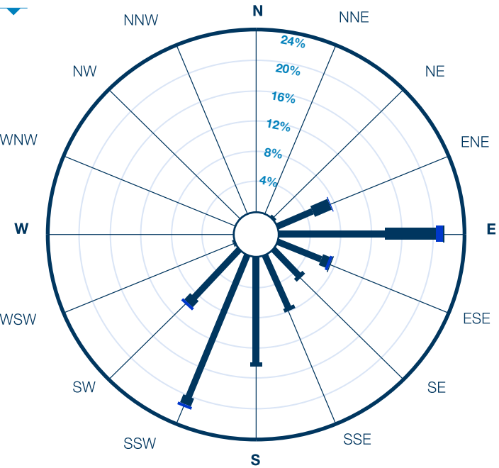
FIG 2: TARIFA BUOY WAVW ROSE
