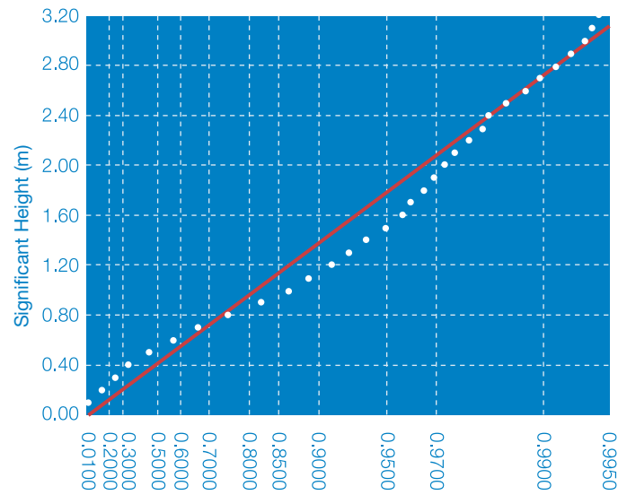
AVERAGE IMPORTANT WAVE HEIGHT SYSTEM
