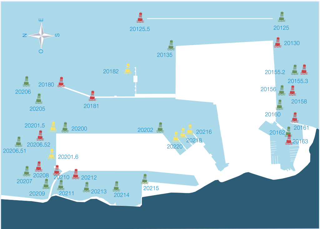
Layout of Algeciras Port marking system
