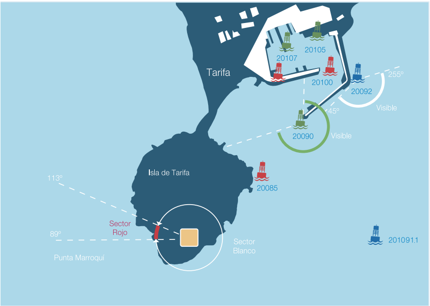
Layout of Tarifa Port and island marking system
