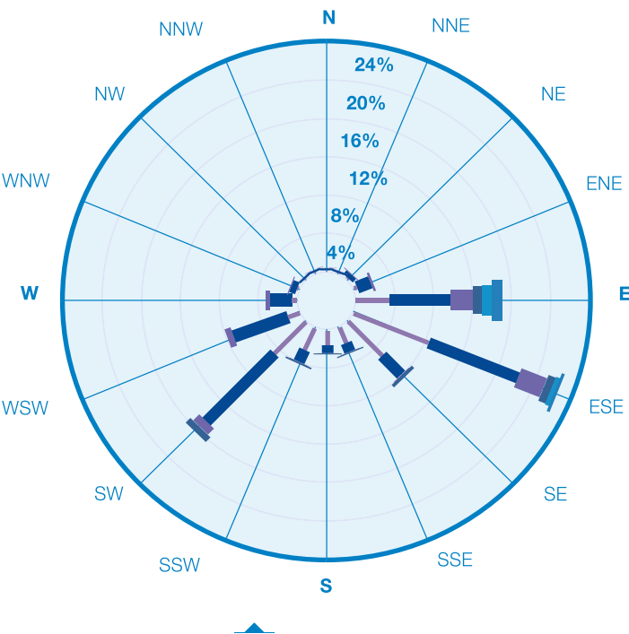
Fig 2: Alboran Sea Buoy wave rose. (Source: State Ports Dept.)
