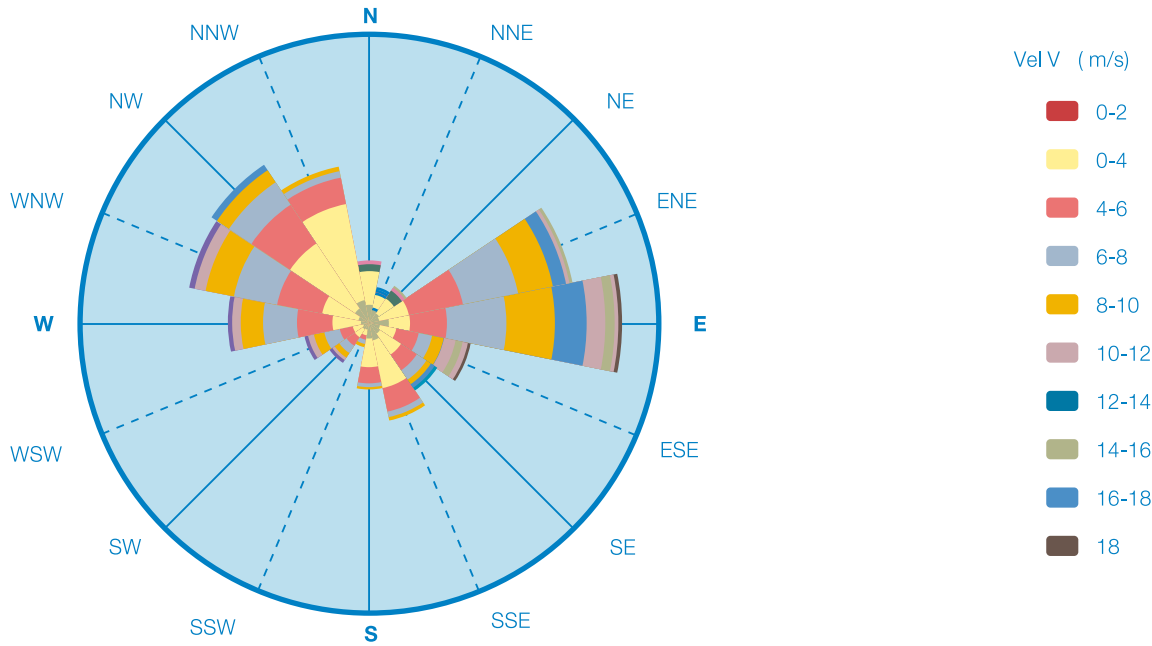
Compass Rose in Port of Algeciras. REMPOR Station (Direction of origin 0=N ; 90=E)
