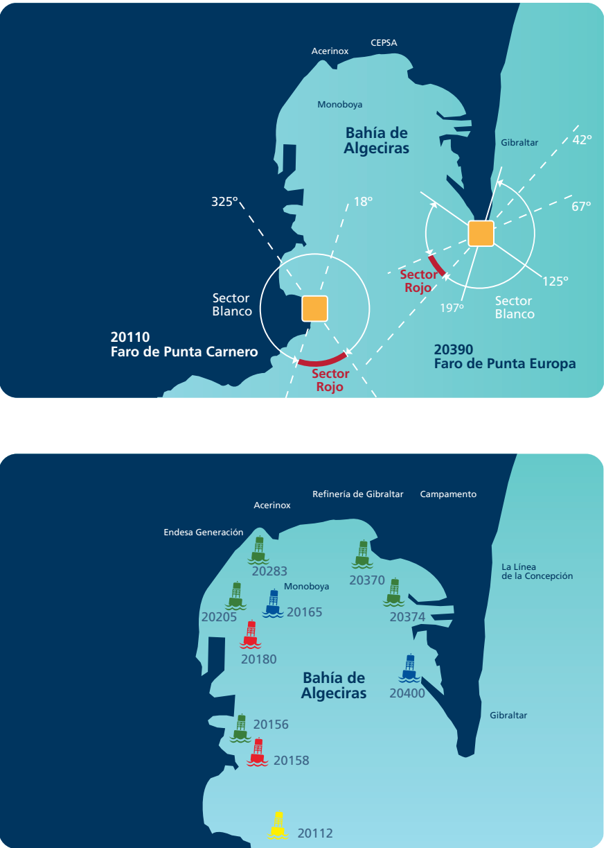
Layout of Bay of Algeciras marking system →
