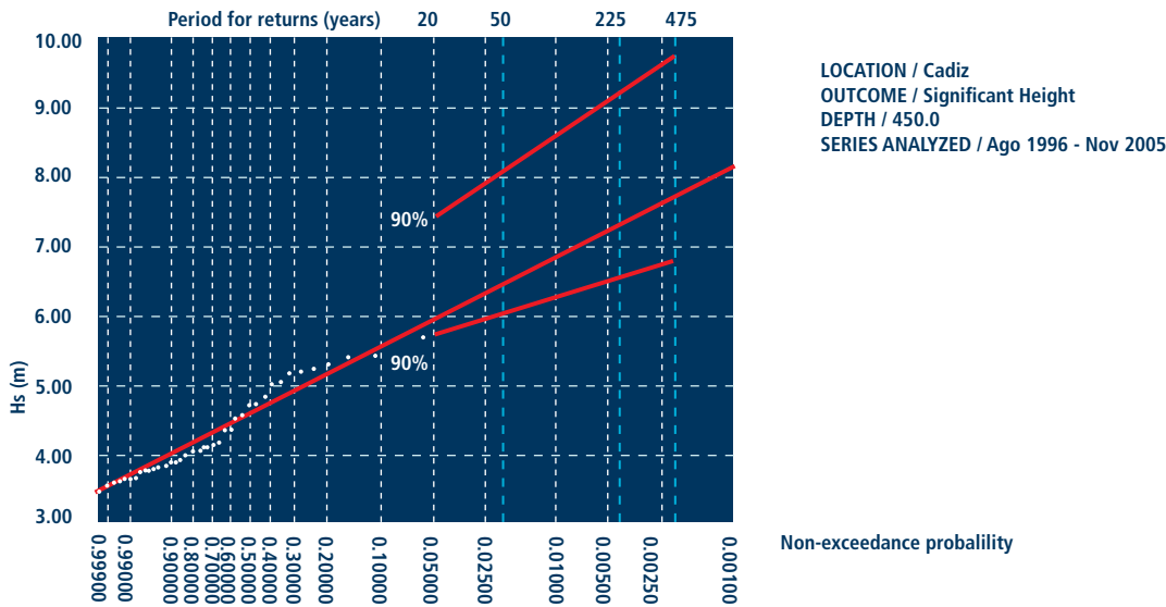
← Fig 8: Board scalar extremal significant wave height in the Gulf of Cádiz buoy.
