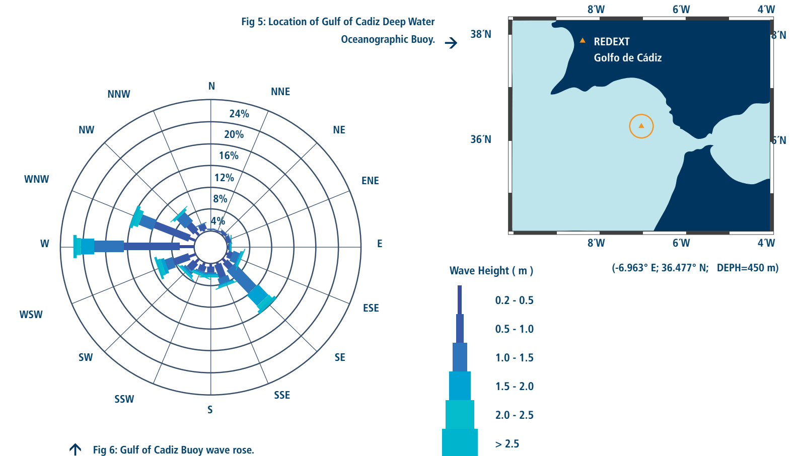
Fig 6: Gulf of Cadiz Buoy wave rose. (Source: State Ports Dept.)
