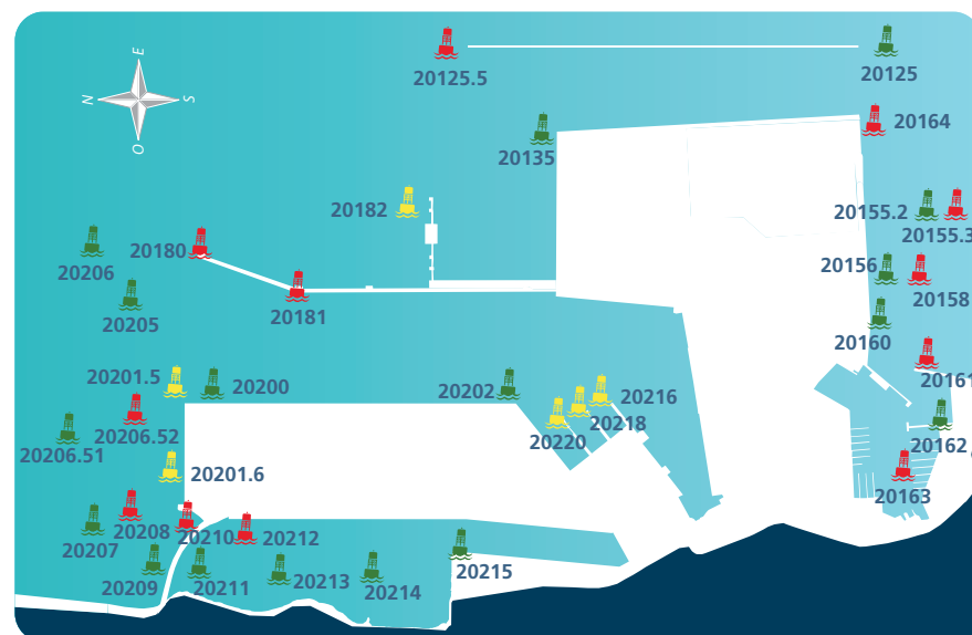
Layout of Algeciras Port marking system →
