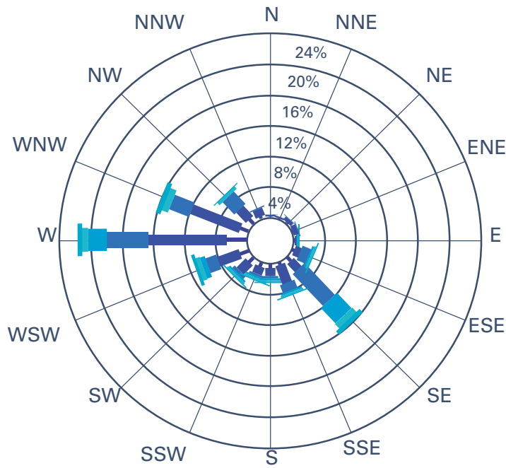
↑ Fig 6: Gulf of Cadiz Buoy wave rose (Source: State Ports Dept.)
