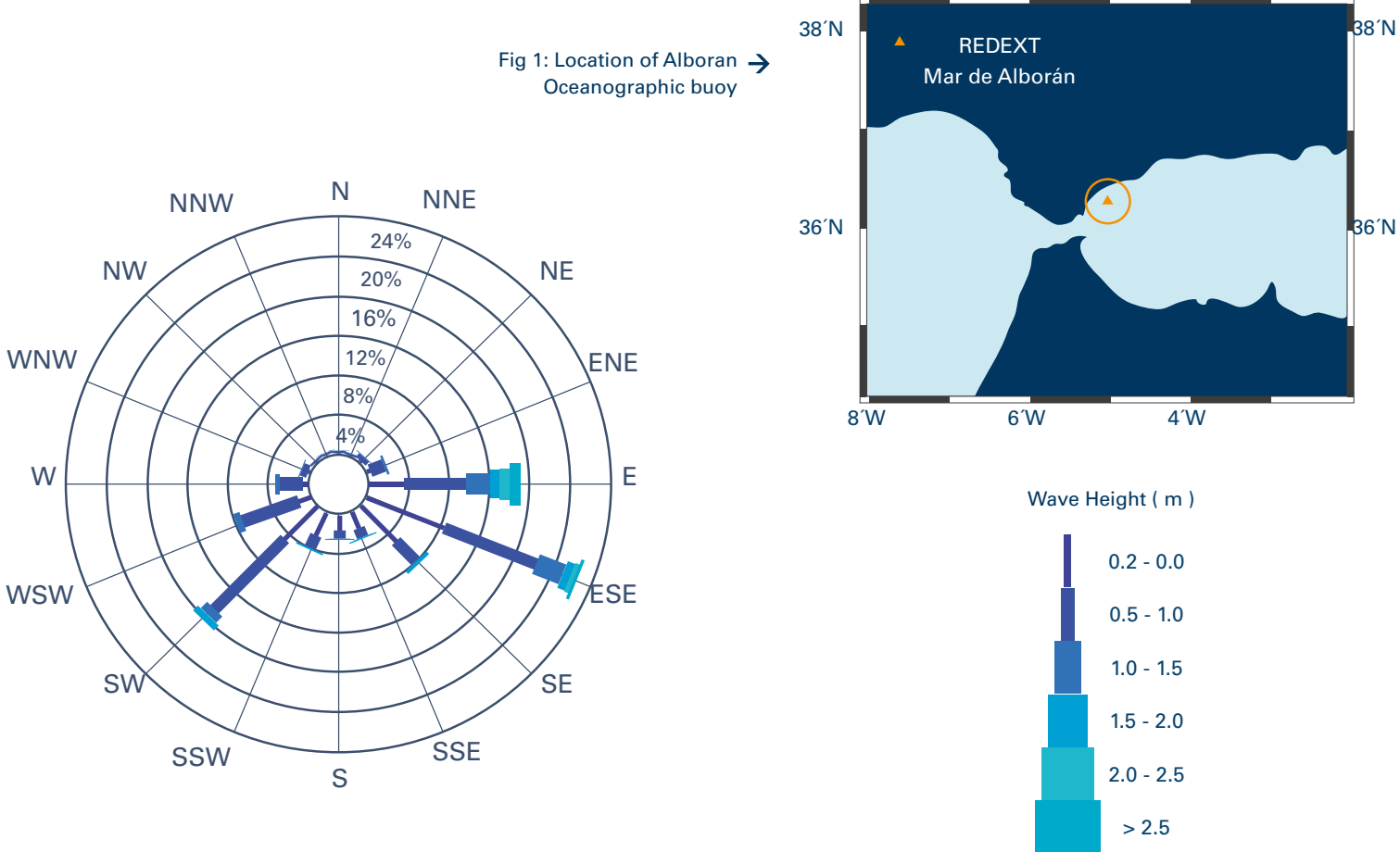
Fig.2: Alboran Sea Buoy wave rose (Source: State Ports Dept.)
