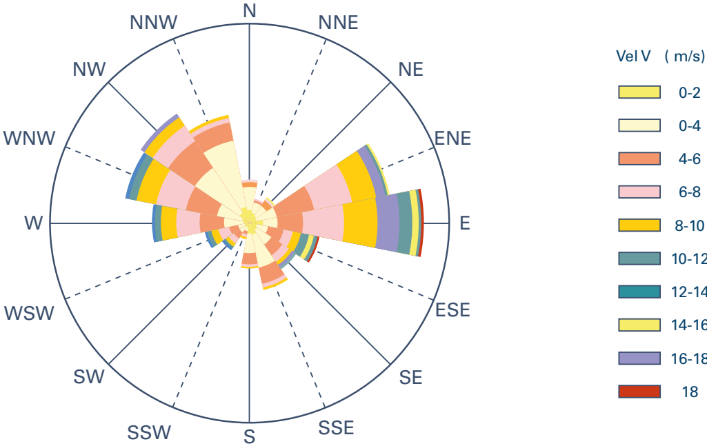
Compass Rose in Port of Algeciras REMPOR Station ( Direction of origin 0=N ; 90=E )
