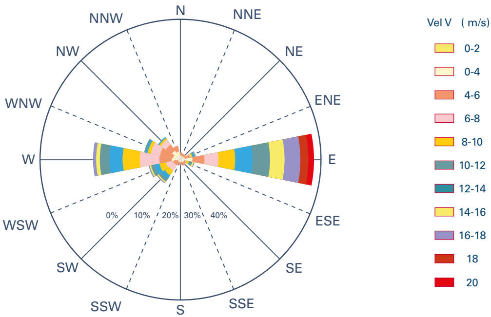
↖ Compass Rose in Tarifa. ( Direction of origin: 0=N ; 90=E )
