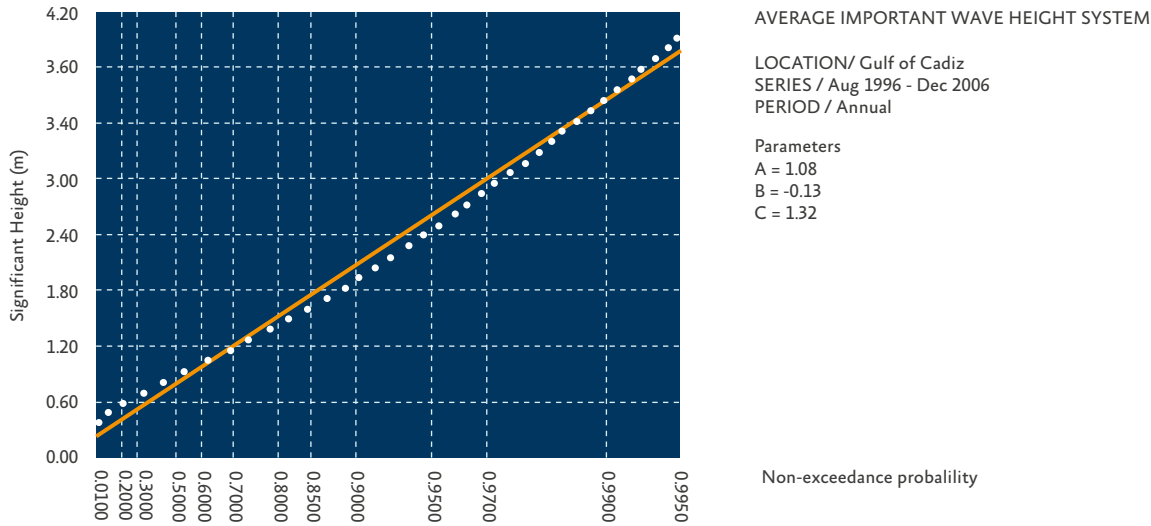
← Fig 7: Average wave climate at Gulf of Cadiz Sea Buoy (Source: State Ports Dept.)
