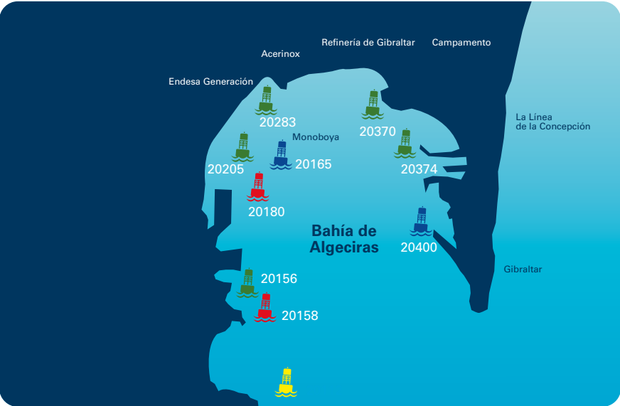
Layout of Bay of Algeciras marking system →
